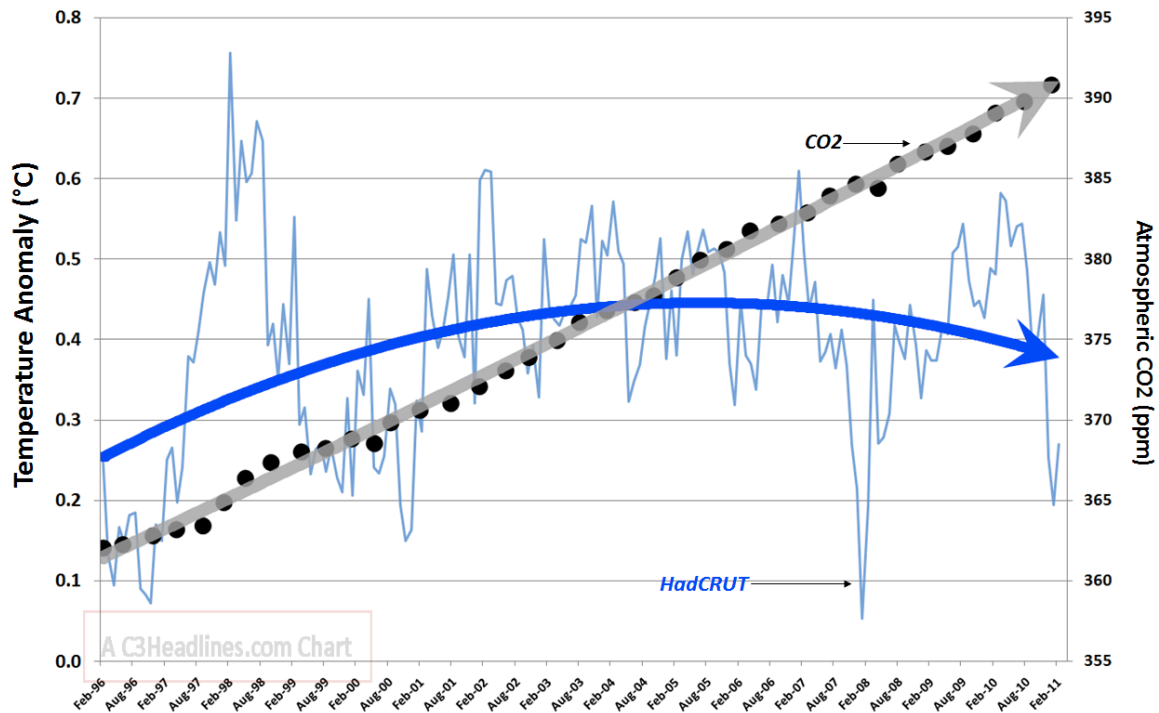
Temperature record from 'HadCRUT' – The Hadley Climate Research Centre (UK) CO2 record from Mauna Loa Observatory , Hawaii
